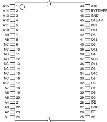
TSOP Type 1
